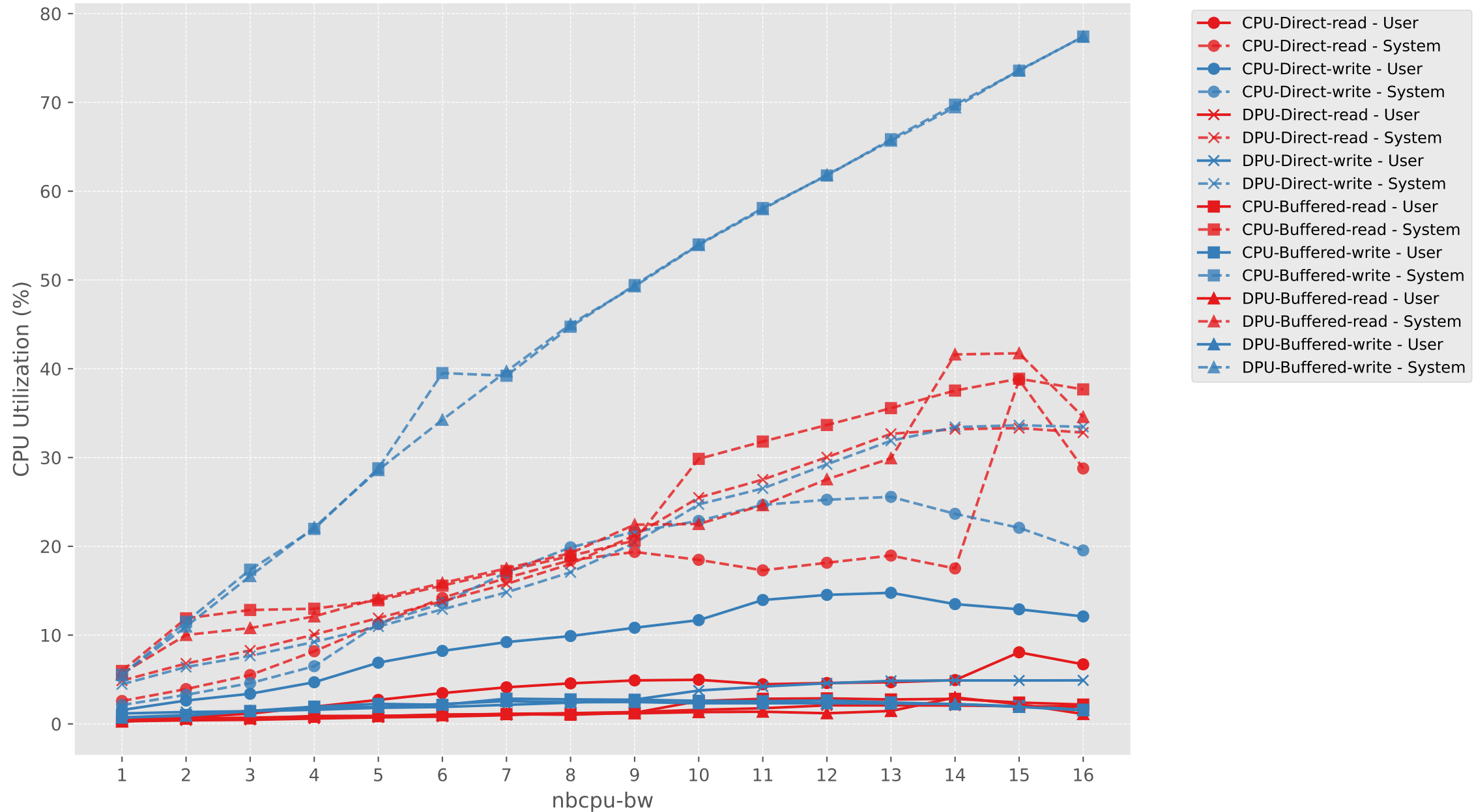
CPU Utilization vs nbcpu-bw (CPU vs DPU, Direct vs Buffered)
